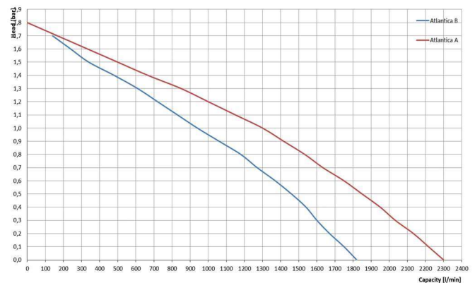
Capacity-head-table
