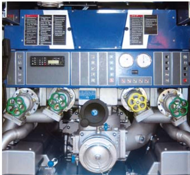
/ The MAGIRUS standard panel was developed according to the specifications of the German fire brigade association DFV and from various customers. The classic alternative.
